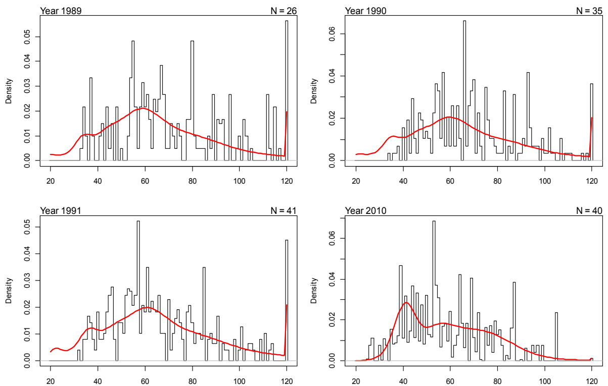
Figure 47: MEC, base, MPD fit to spawning-season age frequencies (N is the assumed effective sample size in the given year). Observations are square-topped black lines; model predictions are the smooth red lines.
