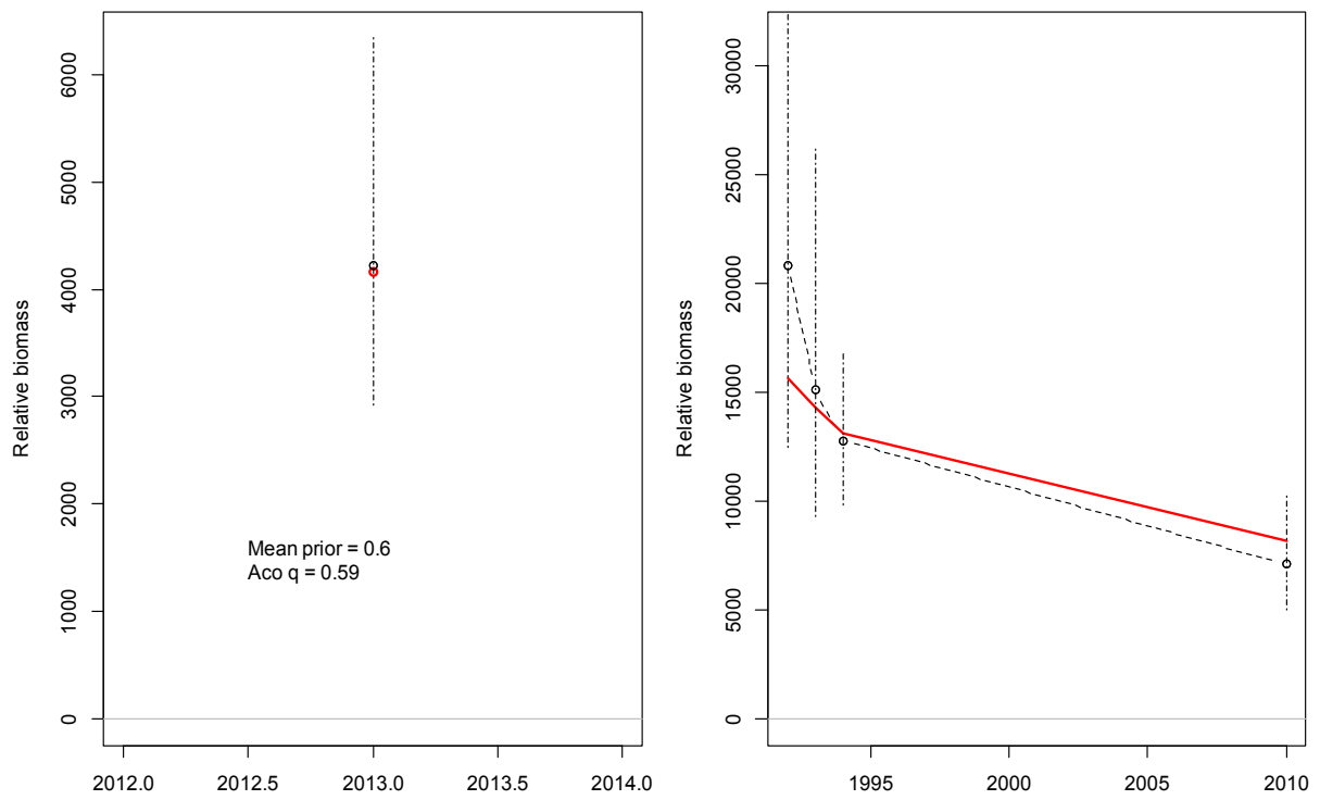
Figure 39: MEC, base, MPD fit to biomass indices: left: acoustic-survey spawning biomass index (fitted with an informed q prior, mean = 0.6; MPD estimated q = 0.59); right: Tangaroa trawl-survey indices. Vertical lines are 95% CIs.
