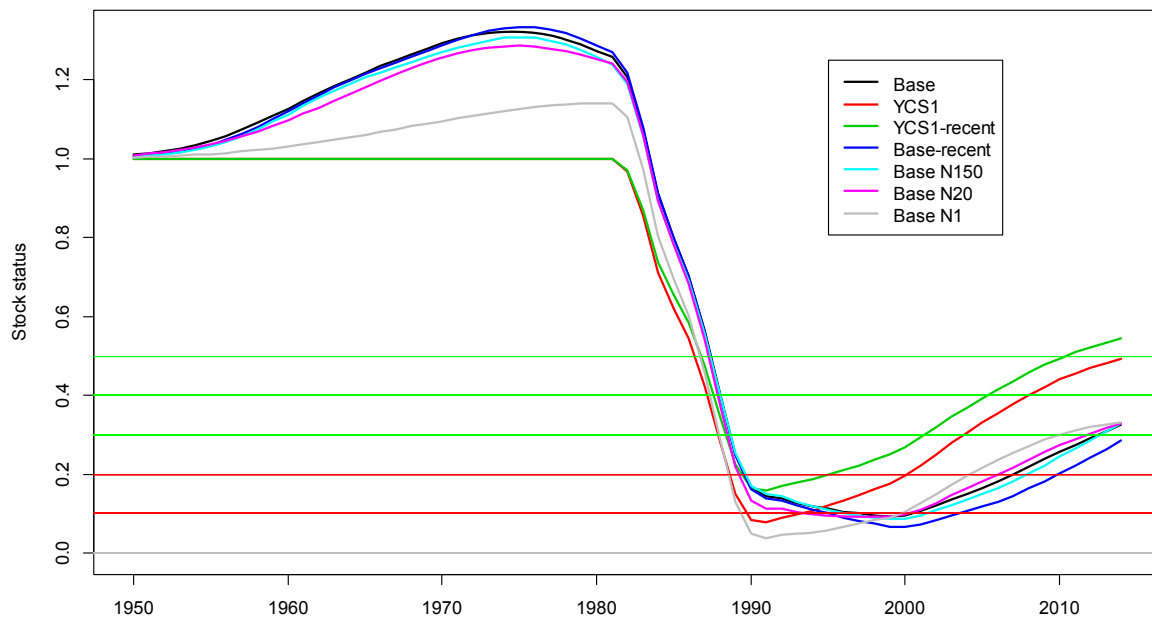
Figure A2.9: ORH7A: MPD stock status trajectory for the base model and some sensitivities: deterministic recruitment with or without recent biomass indices (YCS1, YCS1-recent); the base model without recent biomass indices; alternative effective sample sizes for the age frequency data ( N = 150, 20, 1 ).
