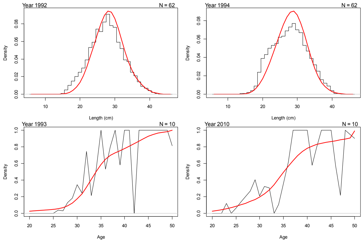
Figure 46: MEC, base, MPD fits to trawl-survey length frequencies (N is the assumed effective sample size in the given year) and proportion spawning-at-age (N =10 is the binomial sample size assumed for each age). Observations are jagged black lines; model predictions are the smooth red lines.
