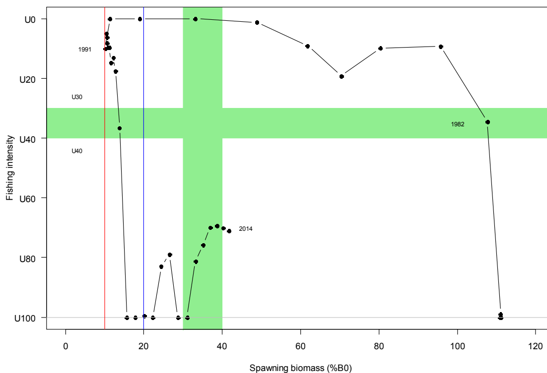
Figure 37: ORH 7A: historical trajectory of spawning biomass ( \%B_0 ) and fishing intensity (%) (base model, medians of the marginal posteriors). The biomass target range of 30–40% B_0 and the corresponding fishing intensity range are marked in green. The soft limit (20% B_0 ) is marked in blue and the hard limit (10% B_0 ) in red.
